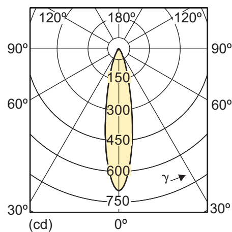
4-35W GU10 WH 25D
