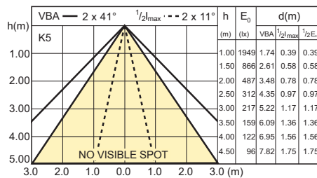
KoD 8-50W GU10 CW 25D 4000K
