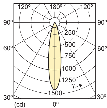
8-50W GU10 WW 25D 2700K Ra=90
