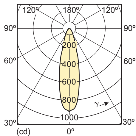
6-50W GU10 WW 25D 2700K
