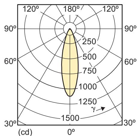
5.5-50W GU10 827 2700K 25D
