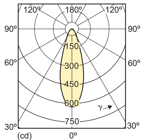
6-50W GU10 CW 40D 4000K
