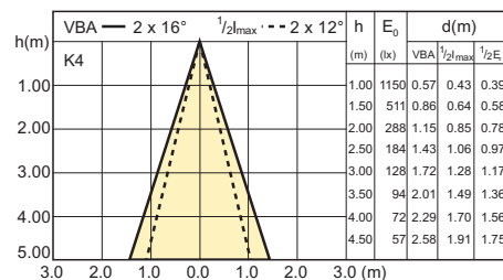
MASTER LED 7-50W GU10 3000K 240V 25D
