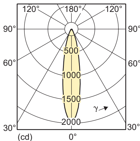
KoD 8-50W GU10 CW 25D 4000K
