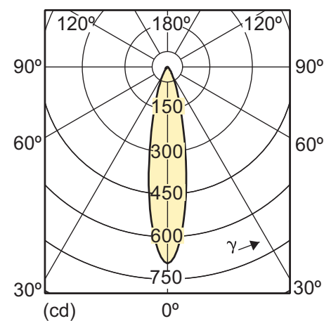
4-35W GU10 WW 40D
