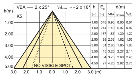
MASTER LEDspotMV 5.5-50W GU10 3000K 40D
