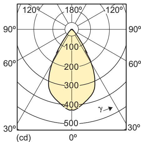
5.5-50W GU10 827 2700K 60D
