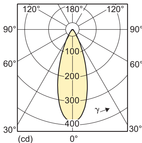
4-35W GU10 CW 40D
