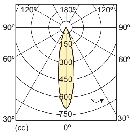
4-35W GU10 WW 25D
