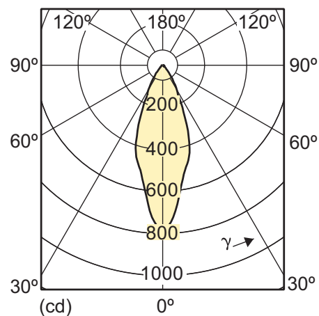
5.5-50W GU10 827 2700K 40D
