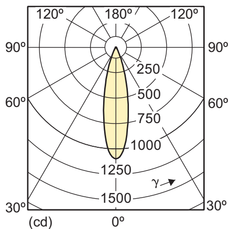
MASTER LEDspotMV 5.5-50W GU10 2700K 25D
