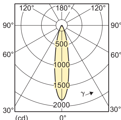
KoD 8-50W GU10 WW 25D 2700K
