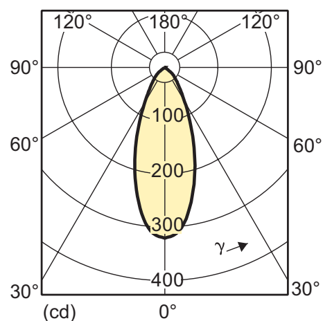
MASTER LED 7-50W GU10 4000K 40D
