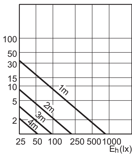
MASTER LEDspotMV 3-35W GU10 2700K 25D
