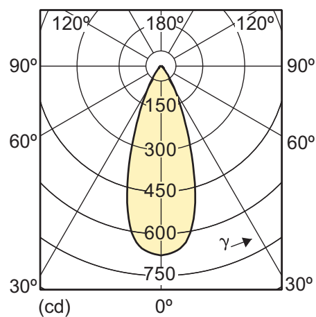
8-50W GU10 WW 40D 2700K Ra=90
