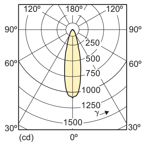
6-50W GU10 WH 25D 3000K
