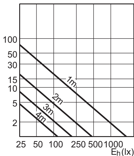
KoD 8-50W GU10 WH 25D 3000K
