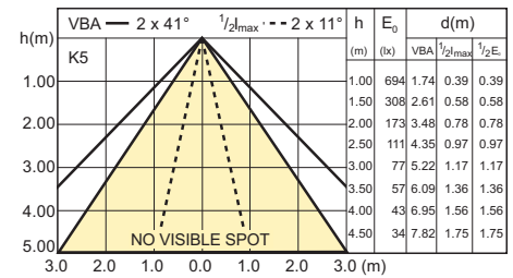
4-35W GU10 WW 40D
