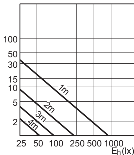
KoD 8-50W GU10 WW 40D 2700K
