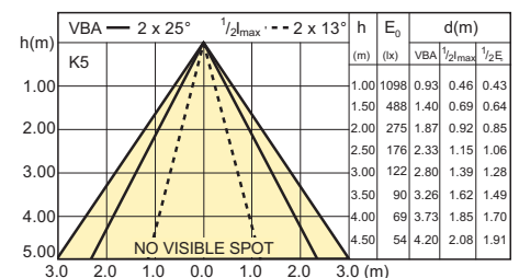
MASTER LEDspotMV 5.5-50W GU10 2700K 25D
