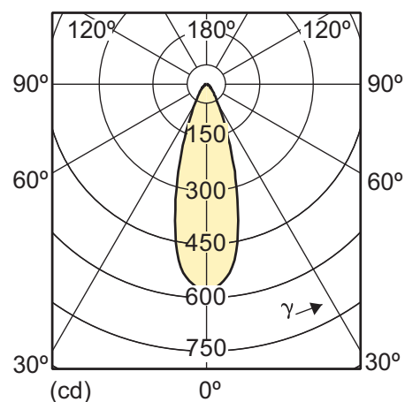
4-35W GU10 827 2700K 40D
