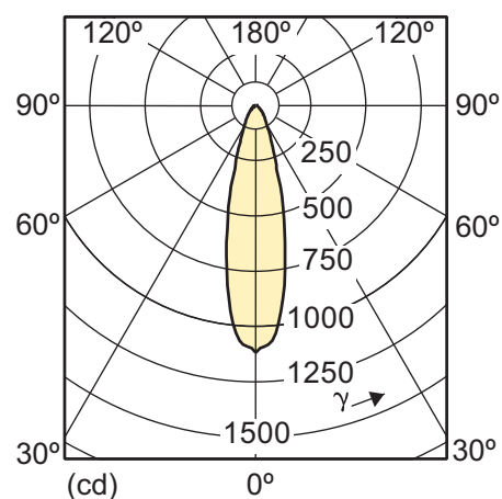
6-50W GU10 CW 25D 4000K
