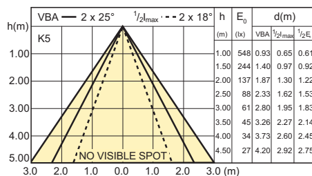
MASTER LEDspotMV 5.5-50W GU10 2700K 40D
