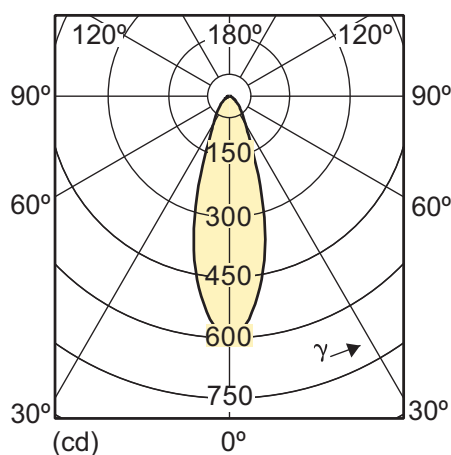
KoD 8-50W GU10 WW 40D 2700K
