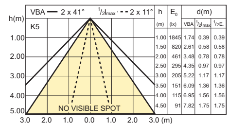
KoD 8-50W GU10 WW 25D 2700K
