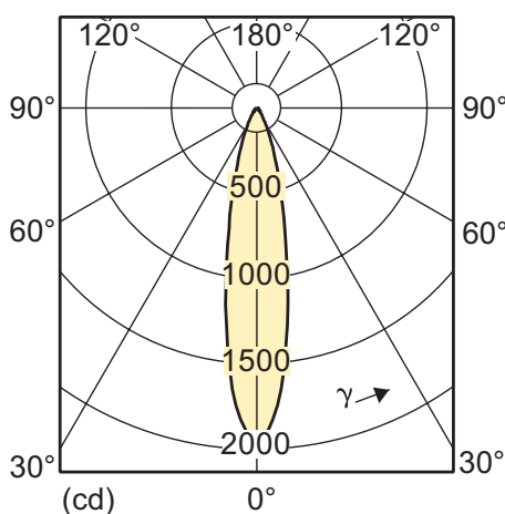
KoD 8-50W GU10 WH 25D 3000K
