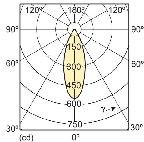
MASTER LEDspotMV 5.5-50W GU10 2700K 40D
