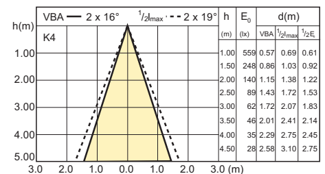
MASTER LED 7-50W GU10 3000K 240V 40D
