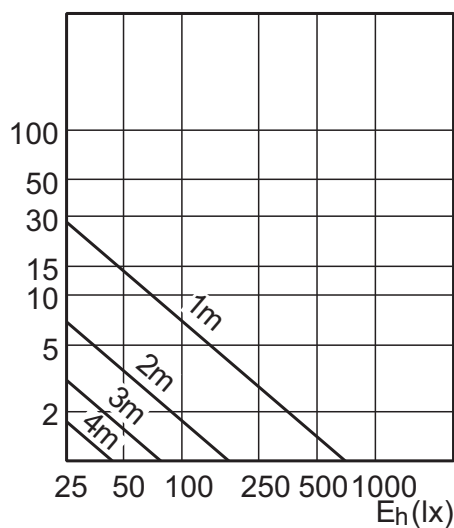
8-50W GU10 WW 40D 2700K Ra=90
