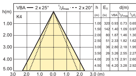
MASTER LED 7-50W GU10 4000K 40D
