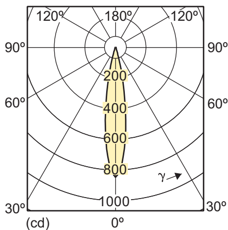
MASTER LEDspotMV 3-35W GU10 2700K 25D
