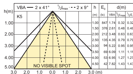
MASTER LEDspotMV 3-35W GU10 2700K 25D
