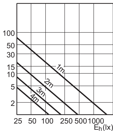
KoD 8-50W GU10 CW 25D 4000K
