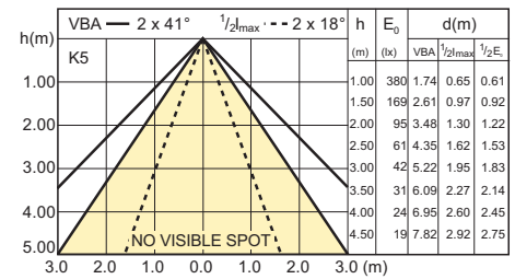
4-35W GU10 CW 40D
