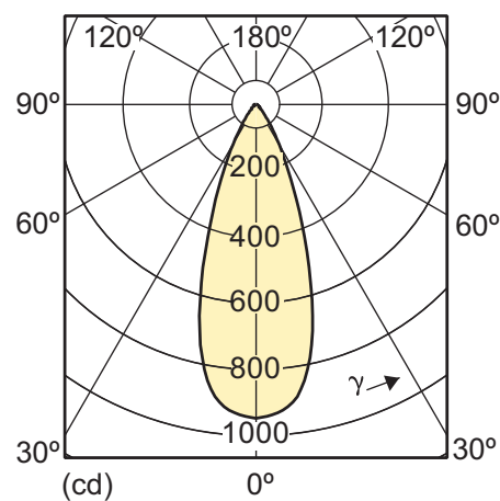
KoD 8-50W GU10 CW 40D 4000K
