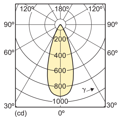
KoD 8-50W GU10 WH 40D 3000K
