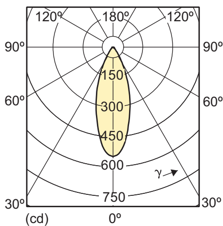
MASTER LEDspotMV 5.5-50W GU10 3000K 40D
