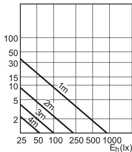
6-50W GU10 WW 25D 2700K
