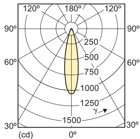
4-35W GU10 827 2700K 25D
