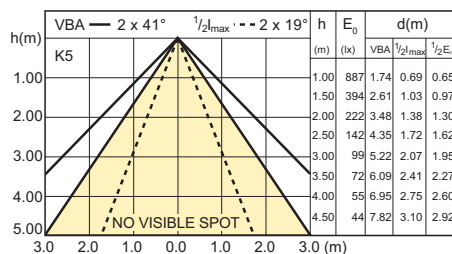
KoD 8-50W GU10 WW 40D 2700K
